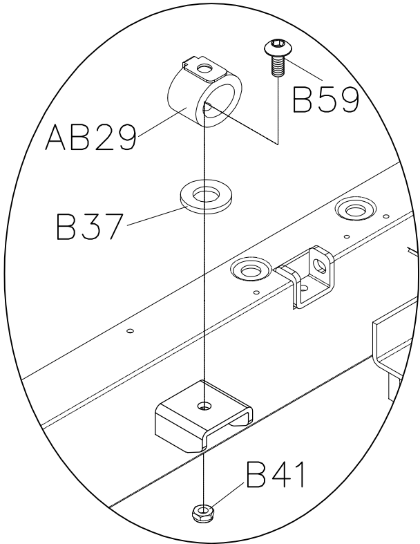
A(1: 5)
